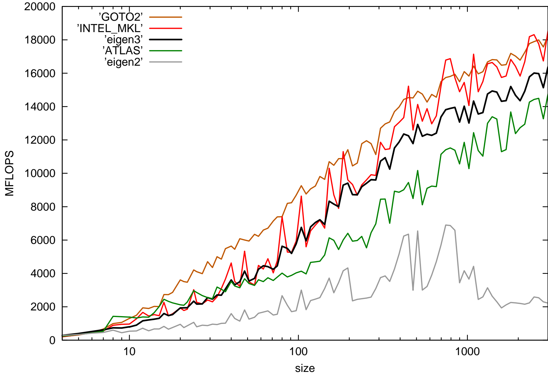
triangular solver - matrix ( M = \text{inv}(L) M )
